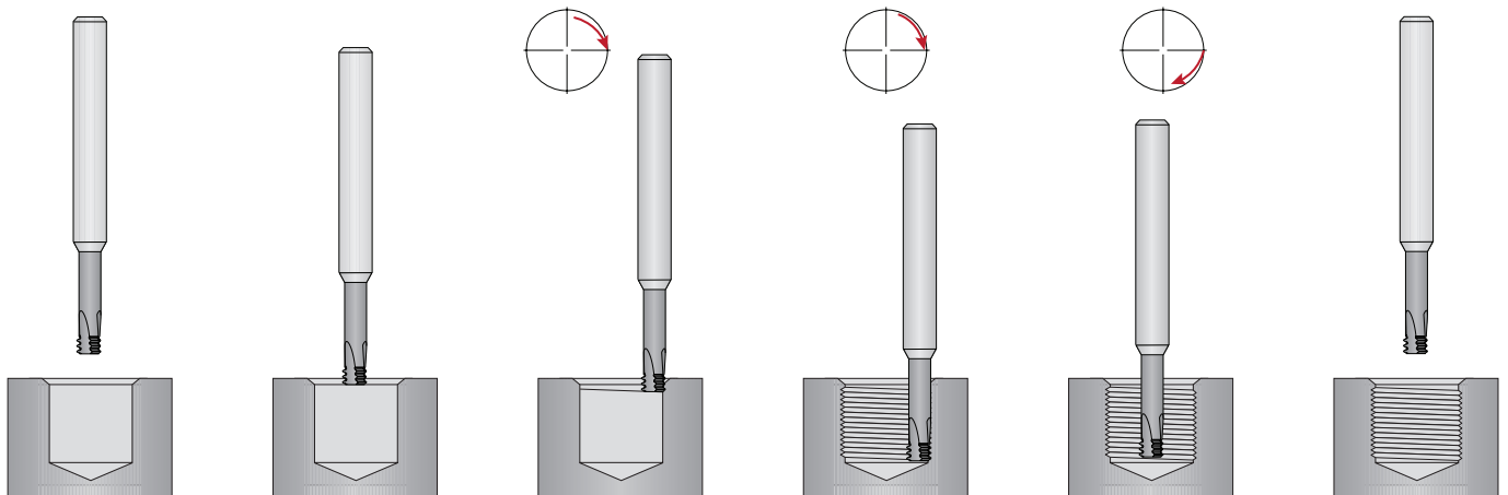
Thread Milling
